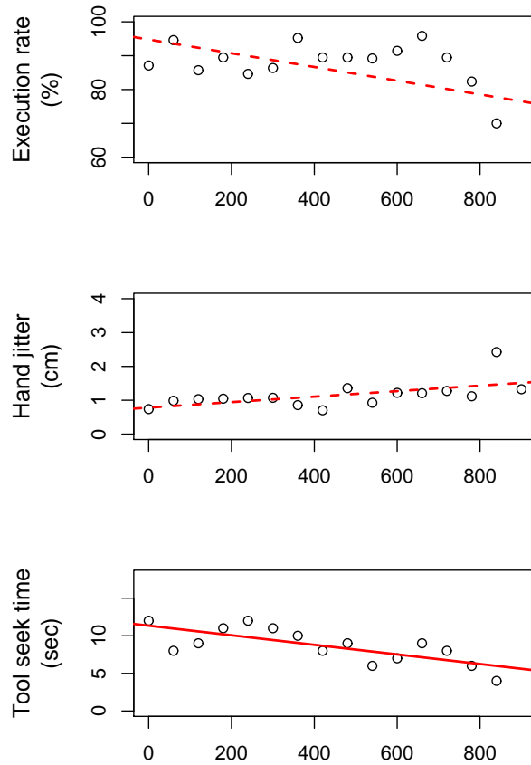
Figure 6: Participants with sliding viewport demonstrated declining learning pattern, hand stability degraded, tool seek times improved from 11.3 seconds to 5.56 seconds. p_{slope} values: 0.0420, 0.0155, 0.00173.
