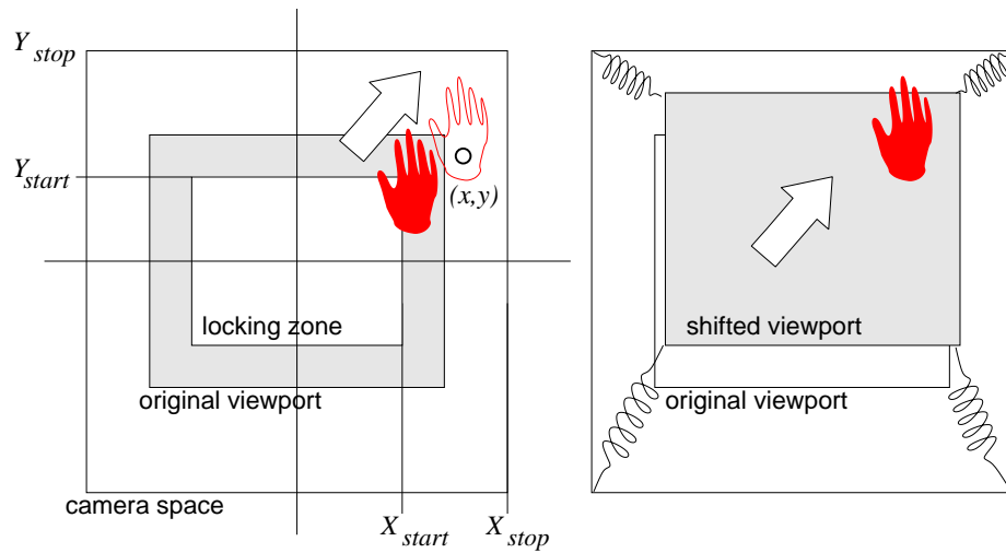
Figure 2: The sliding viewport algorithm computes new positions of the viewport, based upon the current position of the hand in camera space. As a result, the view slides towards the hand, ensuring its continuous visibility.
